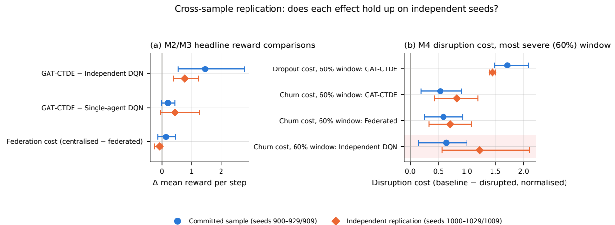
Fig. 7. Every headline paired comparison in this paper, committed sample (seeds 900–929/909) against the independent replication sample (seeds 1000–1029/1009), recomputed from raw logs for both. (a) M2/M3 reward comparisons. (b) M4 disruption cost at the most severe (60%) window. The bottom row of (b), independent DQN’s churn cost, is the one comparison whose two samples visibly disagree on more than point-estimate noise – the finding retracted in Section VIII-D.
