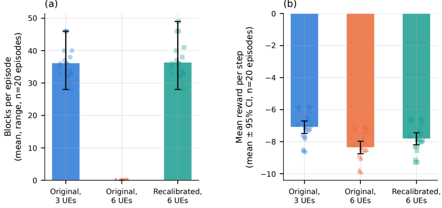
Fig. 8 Three live campaigns, 20 episodes each, real per-slice UDP traffic throughout: the original checkpoint at 3 UEs, the same checkpoint at 6 UEs, and a checkpoint retrained against the recalibrated simulator at 6 UEs. (a) Blocks per episode, mean and range across all 20 episodes – the original checkpoint’s complete silence at 6 UEs sits between two conditions of comparable, healthy block volume. (b) Mean reward per step, mean \pm 95% CI with individual episodes behind it. Block precision (not plotted; one condition is undefined) was 1.000 for both the original-3UE and recalibrated-6UE conditions and undefined (zero blocks) for the original-6UE condition.
