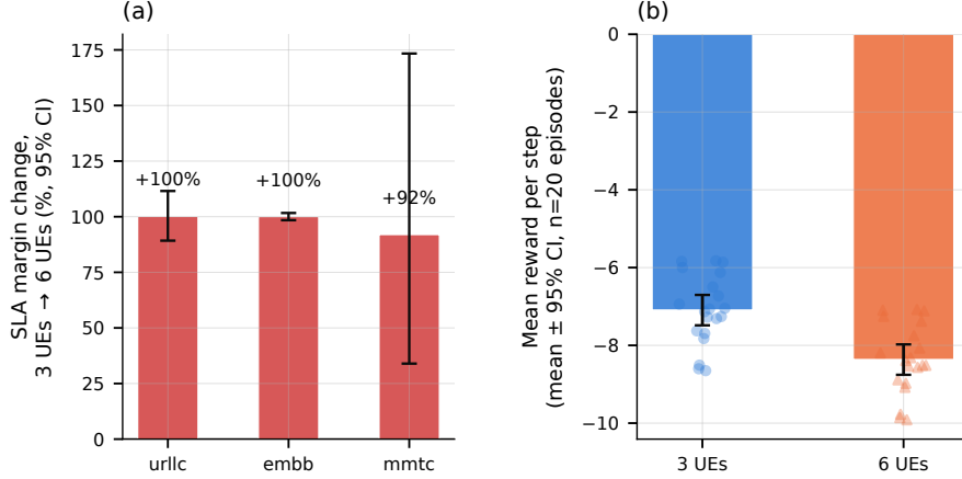
Fig. 7 Live single-gNB comparison, same seed-900 checkpoint, 3 UEs vs. 6 UEs, 20 episodes each, real per-slice UDP traffic throughput. (a) SLA margin percent change per slice from 3 to 6 UEs with 95% bootstrap CI (red: worse) – all three slices worsen substantially. (b) Mean reward per step, mean \pm 95% CI with individual episodes shown behind it – the 6-UE campaign is significantly worse and the intervals do not overlap. Block precision (not plotted, since one side is a single number and the other is undefined) was 1.000 in all 20 episodes at 3 UEs and undefined (zero blocks) in all 20 episodes at 6 UEs.
