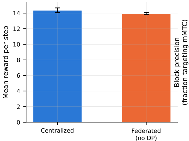
(a) Federation cost (n=10)
