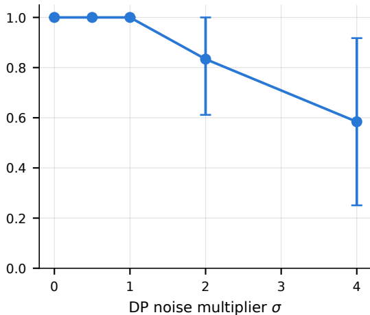
(b) Privacy-utility (block precision)
