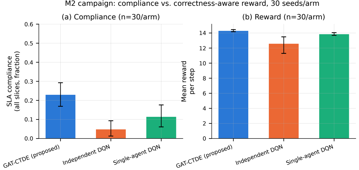
Fig. 3. 30-seed campaign, three arms. (a) The established SLA-compliance metric, where GAT-CTDE’s advantage is present but statistically noisy. (b) Mean reward per step, the correctness-aware metric (Section IV-E): GAT-CTDE’s advantage is tighter and more decisive on the metric that reflects the actual training objective.
