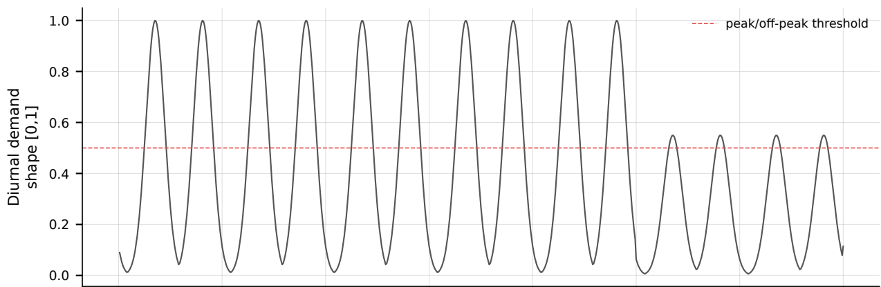
Condensed peak/off-peak week schedule (DQN, SLA reward)
