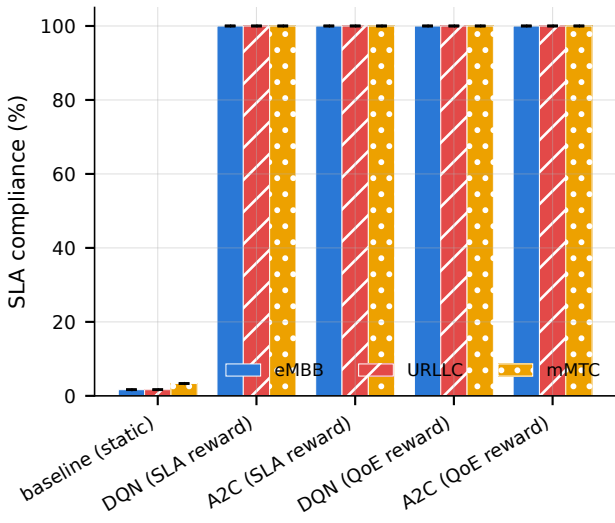
Per-slice SLA compliance by arm
