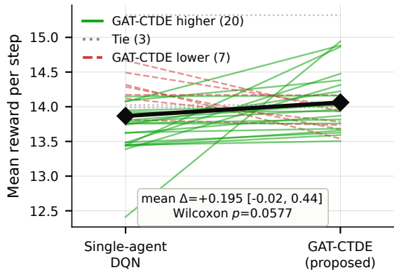
(a) Paired per-seed comparison (n=30)
