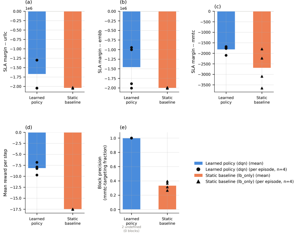
Fig. 7 Live 6-UE comparison, learned single-agent-DQN policy (seed-900 checkpoint) vs. the static lb_only baseline, two independent runs per arm (four episodes total per arm), real per-slice UDP traffic throughout. (a)-(c) SLA margin by slice, one linear axis per slice since the three span orders of magnitude. (d) Mean reward per step: the policy wins every episode. (e) Block precision: perfect (1.000) whenever the policy blocks anything, undefined for the two episodes where it blocked nothing (annotated, not plotted as zero), against the static baseline’s consistently indiscriminate 0.267–0.395.
