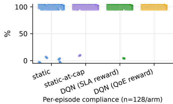
Fig. 4. Per-episode SLA compliance (%), one point per episode.
