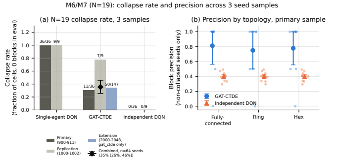
Fig. 8. N = 19 cluster, per-seed evidence across independent seed samples. (a) Collapse rate (fraction of eval runs with zero blocks), pooled across all three topologies. Single-agent DQN collapses totally in every sample; GAT-CTDE’s rate varies sample-to-sample (primary 31%, replication 78%, a 49-seed extension targeted specifically at this question 34%), converging to a combined, seed-level-bootstrapped estimate of 35.4% [25.5%, 45.8%] across all 64 independent seeds (diamond marker, error bar). (b) Block precision by topology, primary sample, non-collapsed seeds only (single-agent DQN has none to show): GAT-CTDE’s non-collapsed seeds are mostly near-ceiling but with a low-precision seed at every topology, while independent DQN sits in a narrow, mediocre band, identical across topologies as expected for an arm that never consumes adjacency.
