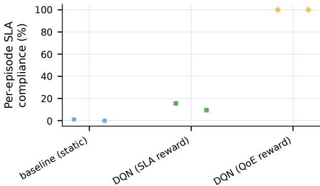
Per-episode SLA compliance by arm (n=2 episodes/arm, seeds=[950])
