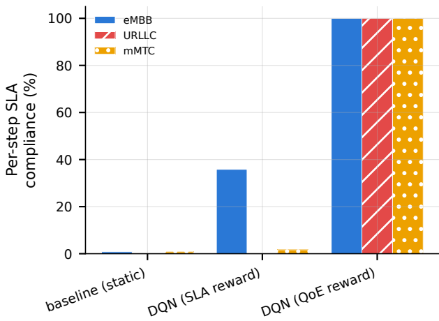
Stage 5 v2 trial (n=2 episodes, seed 950 -- DIRECTIONAL ONLY)
