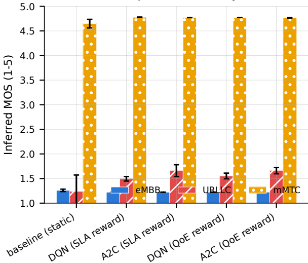
Inferred per-slice MOS by arm
