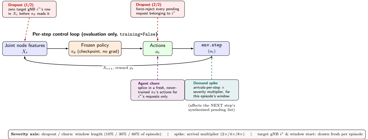
Fig. 6. Where each M4 disruption kind intercepts the frozen policy's per-step evaluation loop. Dropout acts twice (corrupting the target gNB's input row, then separately forcing that gNB's own requests to reject, so a policy cannot simply learn around the corrupted feature); agent churn substitutes a fresh, never-trained policy's actions for the target gNB only, leaving every other agent's decisions untouched; demand spike is entirely external to the policy, acting on the arrival process the environment synthesises for the following step. All three are evaluation-only perturbations - the policy itself is never updated.
