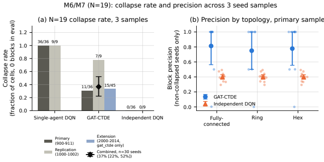
Fig. 8. N = 19 cluster, per-seed evidence across independent seed samples. (a) Collapse rate (fraction of eval runs with zero blocks), pooled across all three topologies – single-agent DQN collapses totally in every sample; GAT-CTDE’s rate varies sample-to-sample (primary 31%, replication 78%, a 15-seed extension targeted specifically at this question 33%), converging to a combined, seed-level-bootstrapped estimate of 36.7% [22.2%, 52.2%] across all 30 independent seeds (diamond marker, error bar). (b) Block precision by topology, primary sample, non-collapsed seeds only (single-agent DQN has none to show): GAT-CTDE’s non-collapsed seeds are mostly near-ceiling but with a low-precision seed at every topology, while independent DQN sits in a narrow, mediocre band, identical across topologies as expected for an arm that never consumes adjacency.
