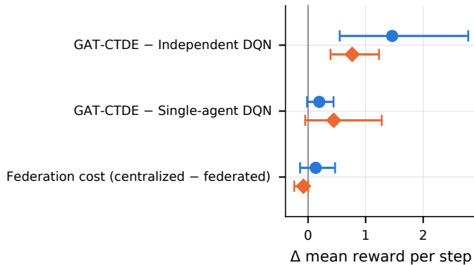
(a) M2/M3 headline reward comparisons
