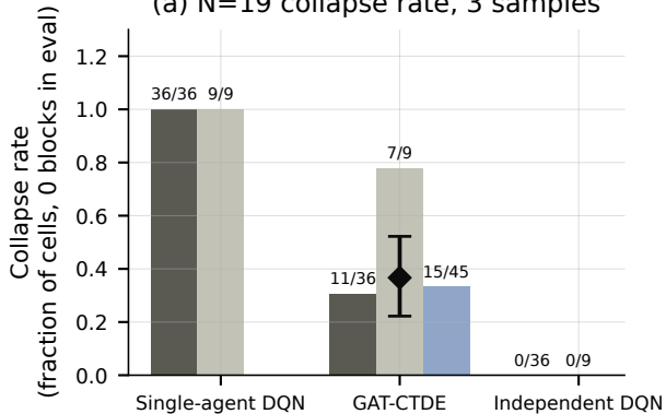
(a) N=19 collapse rate, 3 samples
