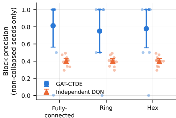
(b) Precision by topology, primary sample
