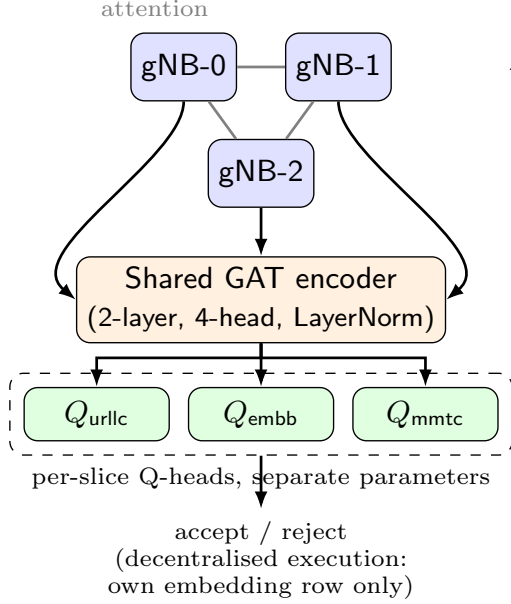
Fig. 1. GAT-CTDE architecture. (a) A shared Graph Attention encoder over the fully-connected 3-gNB topology produces one embedding per node; per-slice Q-heads, each with its own parameters, consume that node’s own embedding row at action-selection time (decentralised execution). (b) The federated training variant: each gNB is a client with a private copy of the same network, synchronised via periodic FedAvg with an optional per-client DP-SGD clip-and-noise step.
