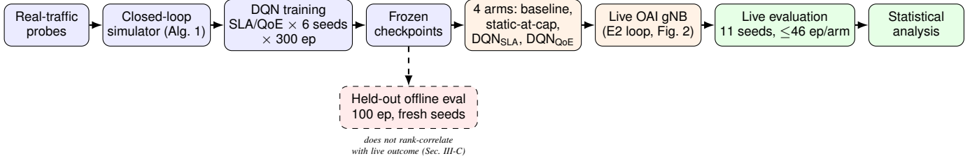
Fig. 1. End-to-end methodology. Real-traffic probe measurements calibrate the offline simulator (Section III-C, Algorithm 1); DQN training produces frozen checkpoints for both reward variants, joined by the two static arms into the four compared conditions, deployed live with no further learning; live episodes are logged and reduced to Table II/Figs. 4–3 via Fisher exact tests and MOS. A held-out offline evaluation runs alongside this live pipeline but, per Section III-C, does not predict its outcome.
