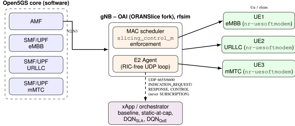
Fig. 2. Testbed software architecture. Open5GS core (AMF, per-slice SMF/UPF) over N2/N3 to an OAI gNB (ORANSlice fork, simulated radio channel) whose MAC scheduler enforces the per-slice ceiling; three nr-uesoftmodem UEs, one per slice, connect over the simulated Uu interface. The RIC-free E2 agent exchanges UDP INDICATION/CONTROL messages (no SUBSCRIPTION channel) with the xApp/orchestrator that all four compared arms run through.
