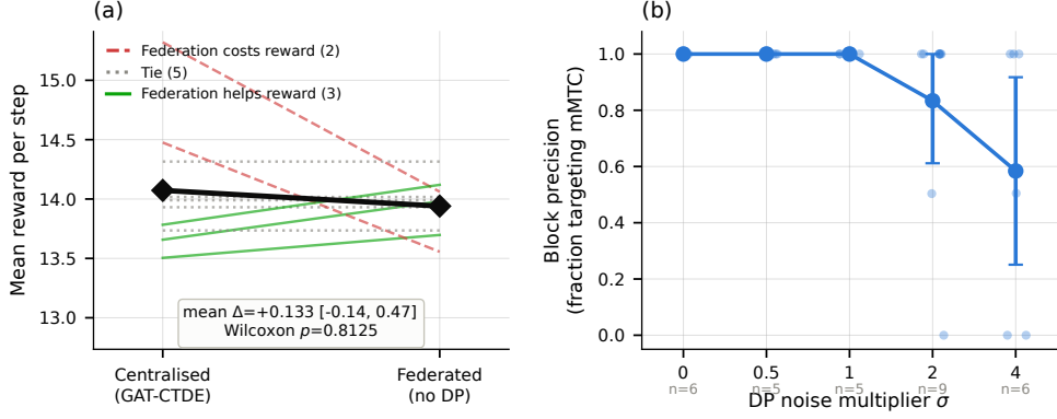
Fig. 3 M3 federated and differential-privacy sweep, per-seed evidence. (a) Paired per-seed federation cost on mean reward per step, same 10 seeds. Centralised scores higher on 2 seeds, federated on 3, 5 ties, no measurable difference (Wilcoxon p = 0.8125 ). (b) Privacy-utility curve using block precision against the DP noise multiplier \sigma , individual seed values (light dots) behind the mean, with the seed count that ever blocked anything at each \sigma printed below (precision is undefined otherwise). Precision is perfect through \sigma = 1.0 , dropping sharply by \sigma = 4.0 .
