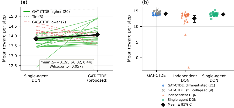
Fig. 2 M2 centralised campaign, per-seed evidence for the correctness-aware metrics (Section 4.4). (a) Paired per-seed comparison against single-agent DQN on mean reward per step. Each line is one seed, coloured by whether GAT-CTDE scored higher (green, 20), tied (grey, 3), or lower (red, 7), the source of this figure’s borderline p = 0.0577 . (b) Full per-seed reward distribution for all three arms. GAT-CTDE is split into seeds that learned genuine differentiated shedding (blue, 21) versus seeds still stuck at the always-accept collapse (grey \times , 9), shown without claiming the split predicts reward, since several still-collapsed seeds score among the arm’s highest.
