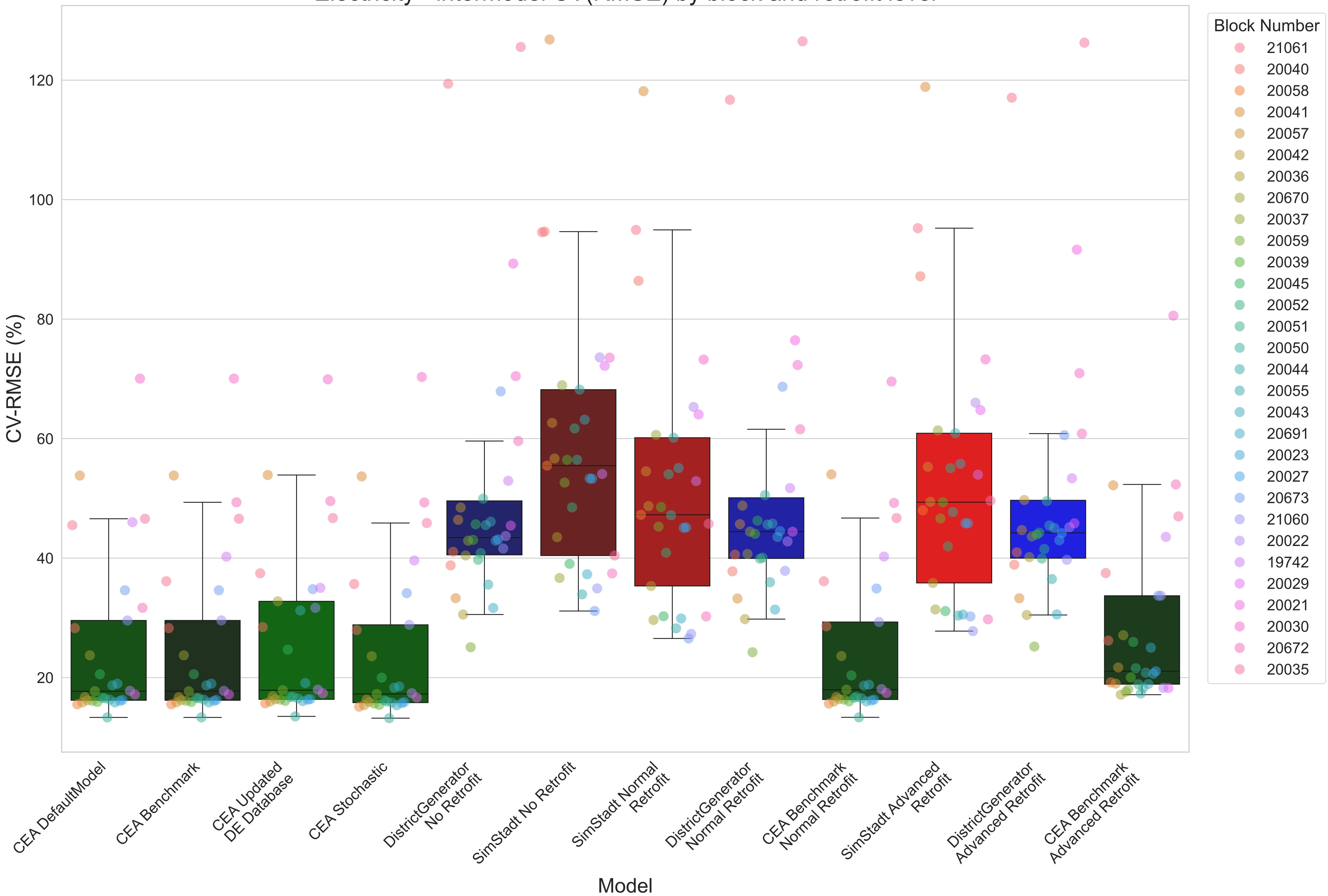
Electricity - intermodel CV(RMSE) by block and retrofit level
