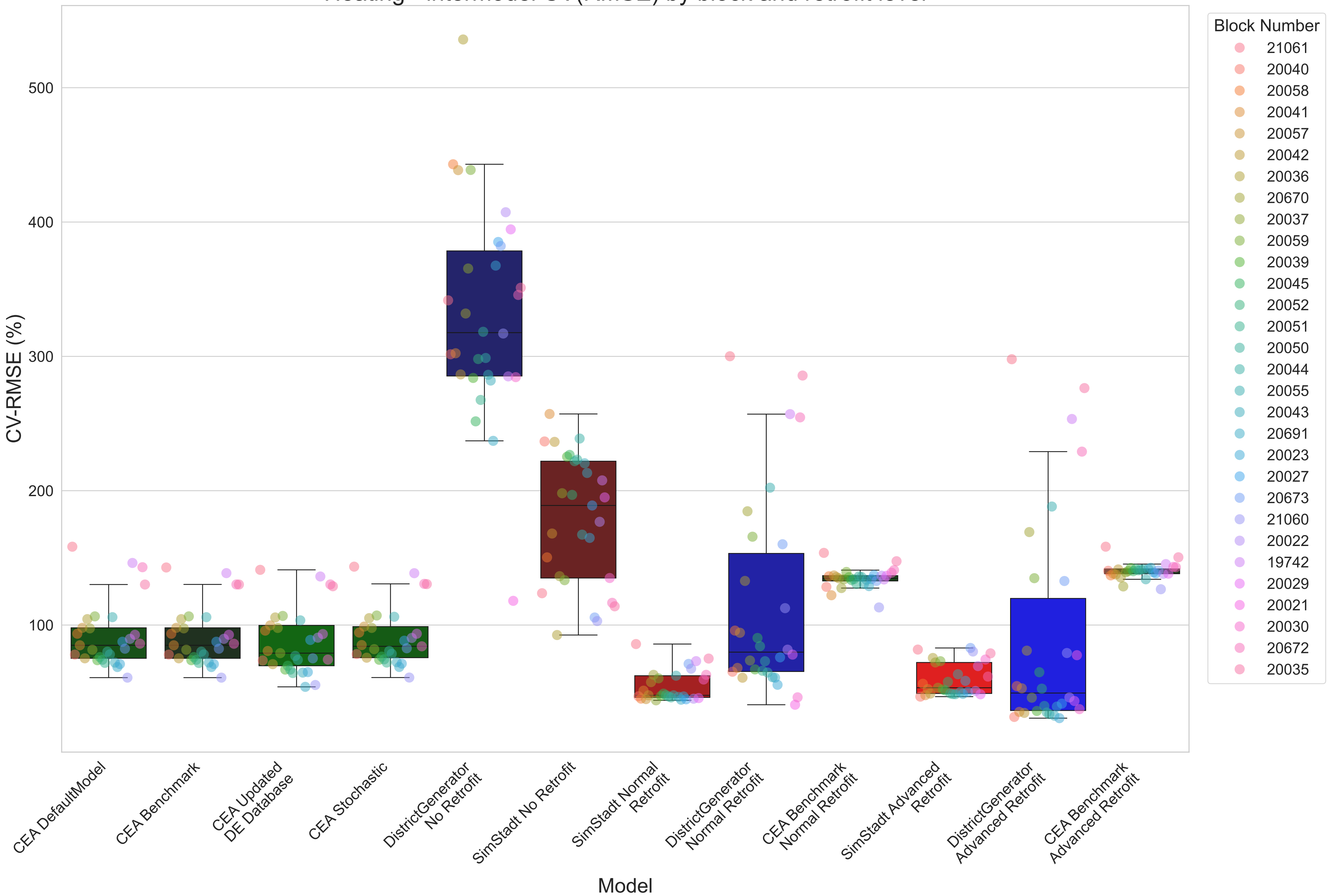
Heating - intermodel CV(RMSE) by block and retrofit level
