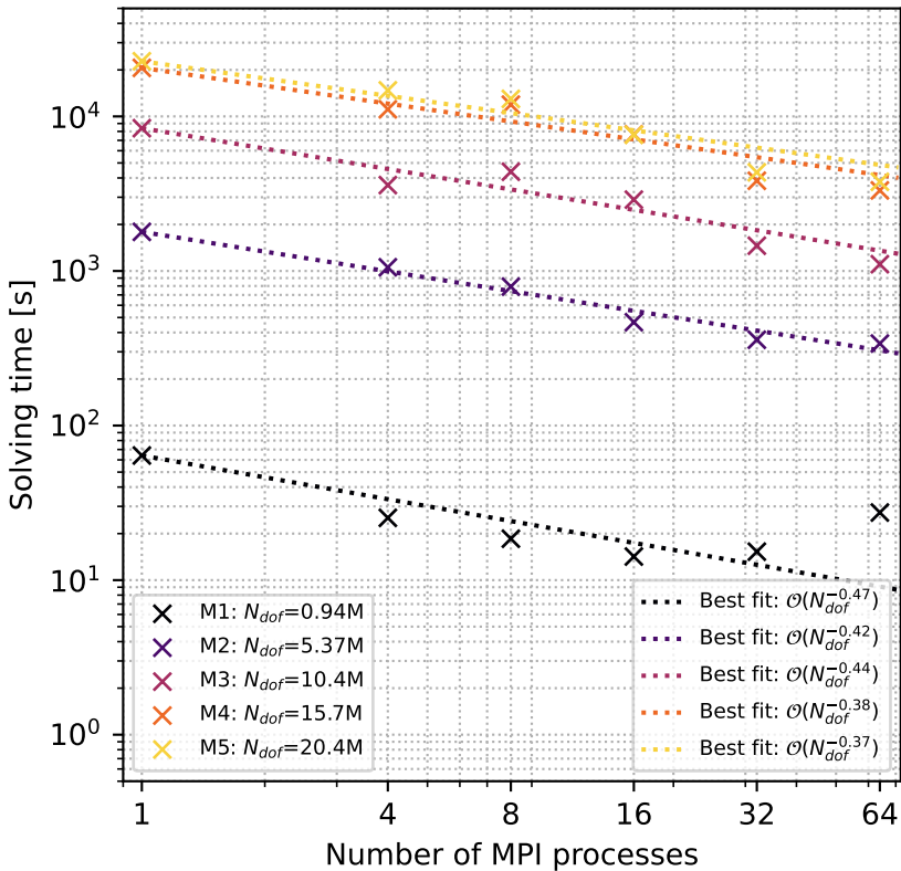
Parallel performance of the direct solver
