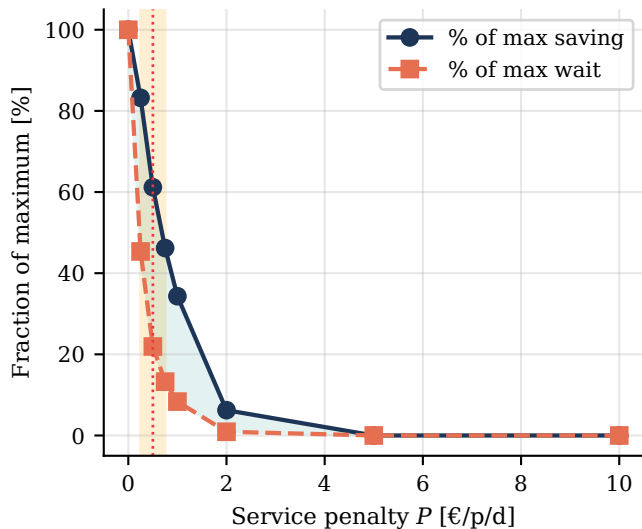
(b) Diminishing returns
