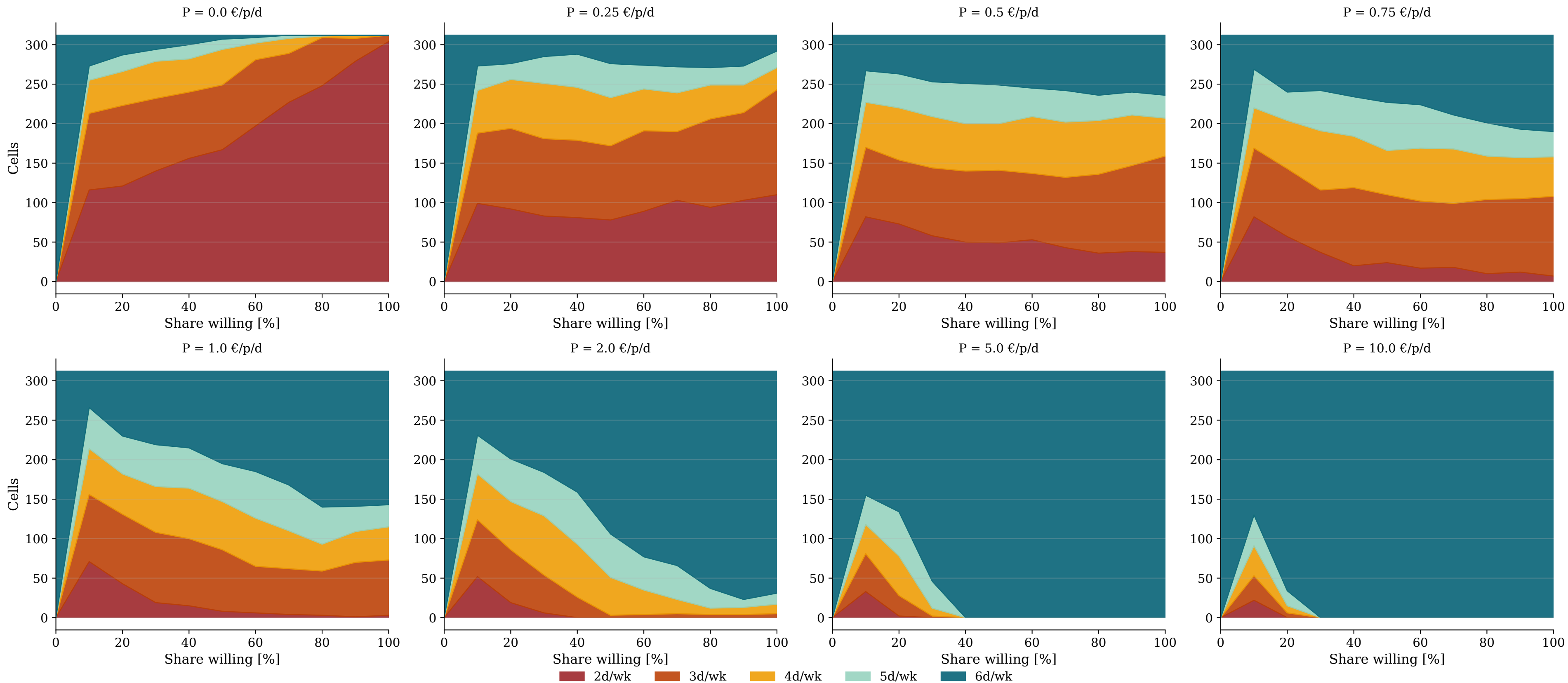
Schedule-size distribution — COST-OPTIMAL (init, no fleet sweep)
