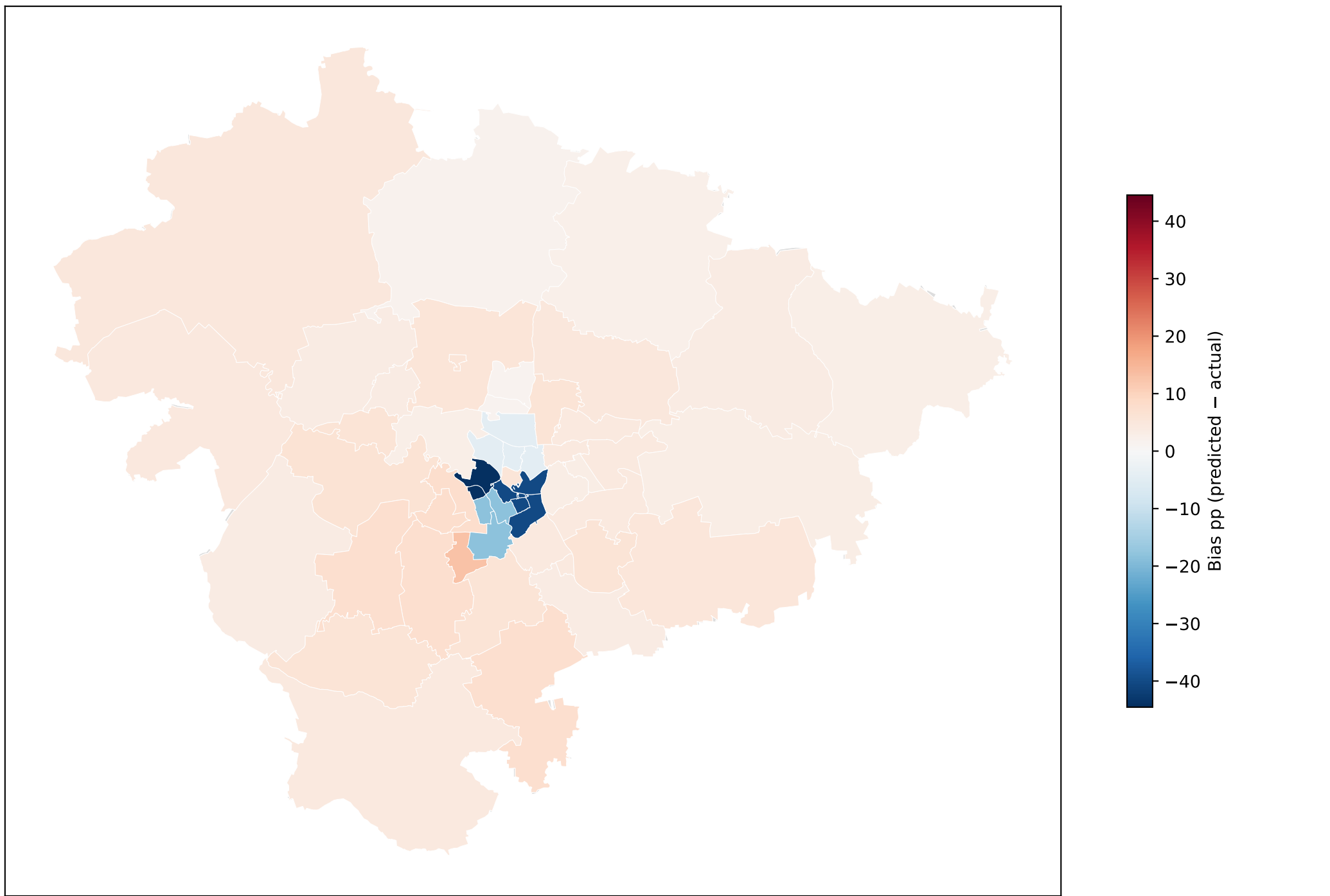
Fig M02 — Saving-prediction bias (LGB-logT – VROOM) per cluster Red = ML overestimates saving; Blue = underestimates. Mean bias +10 pp = Best-of-K winner's curse.
