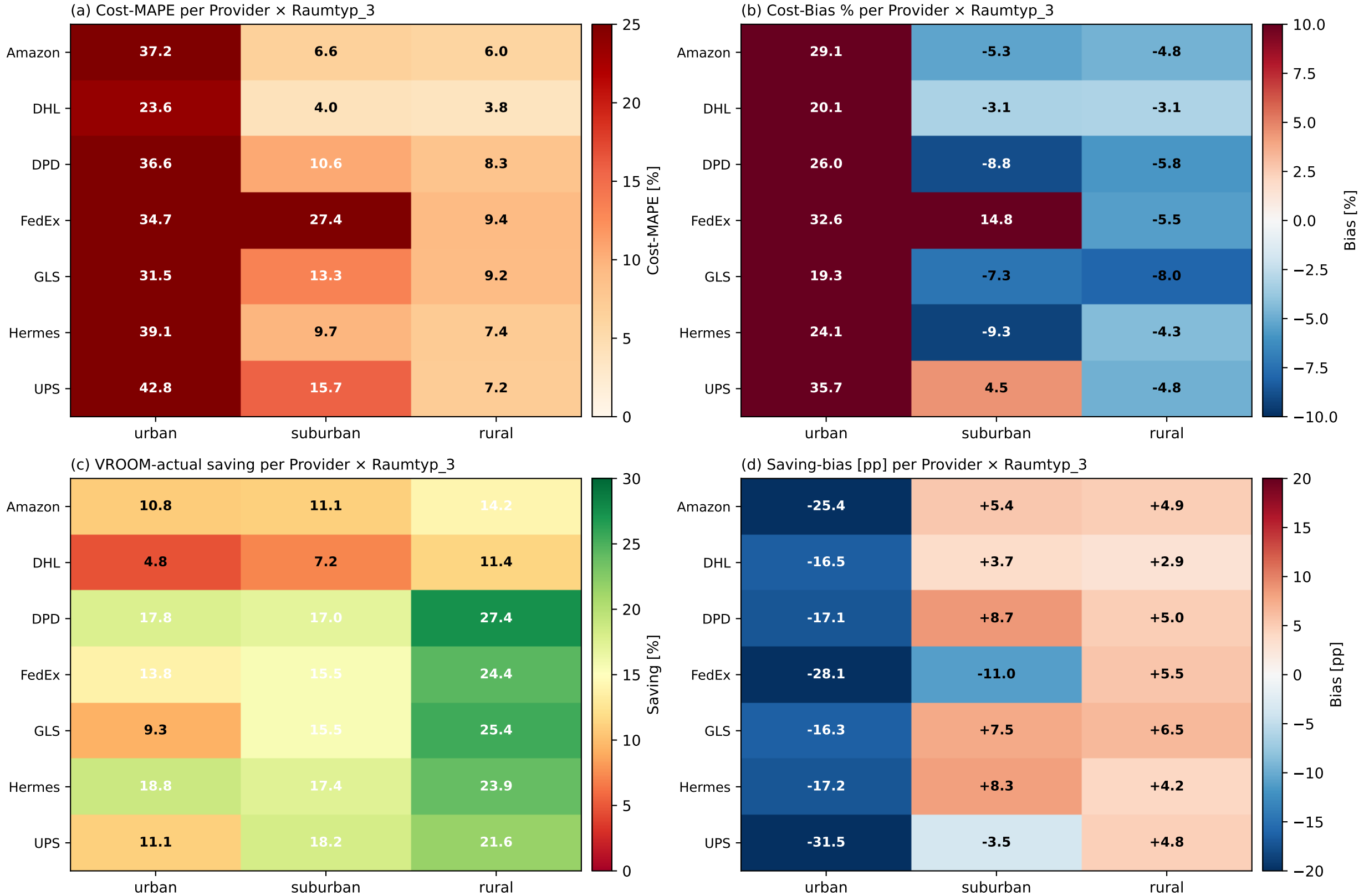
Fig MLA2 — ML accuracy heatmaps: Provider × Raumtyp_3
