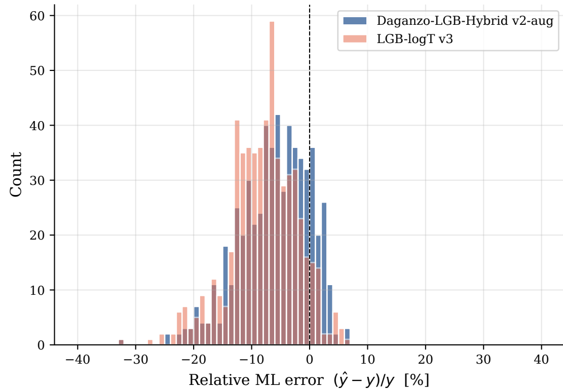
Relative residuals on optimized scenarios
