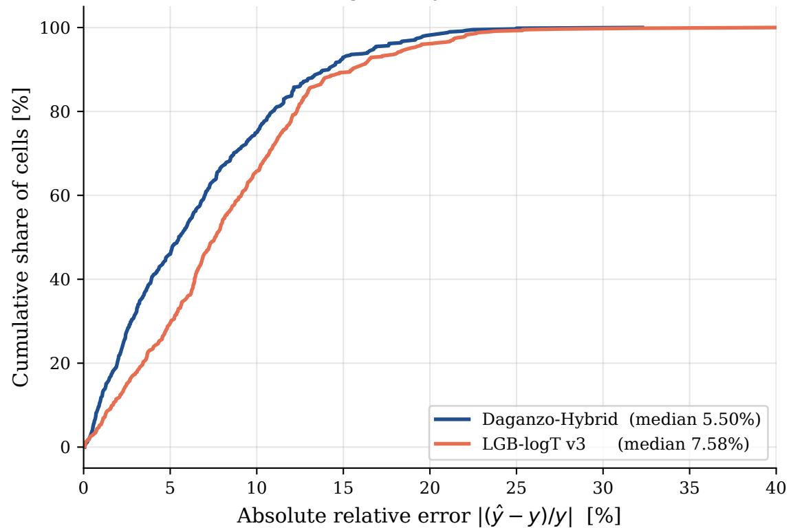
Error CDF — Daganzo-Hybrid dominates LGB-v3
