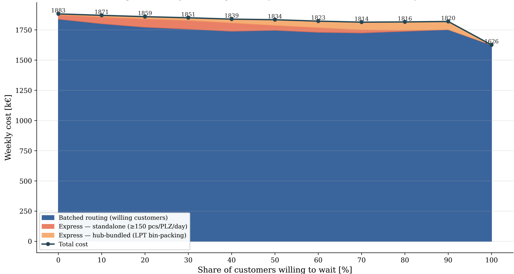
Cost breakdown by service component at P = 0.5 €/parcel/day (Daganzo-LGB-Hybrid surrogate, 312 (provider, PLZ) cells, hub-bundled express)
