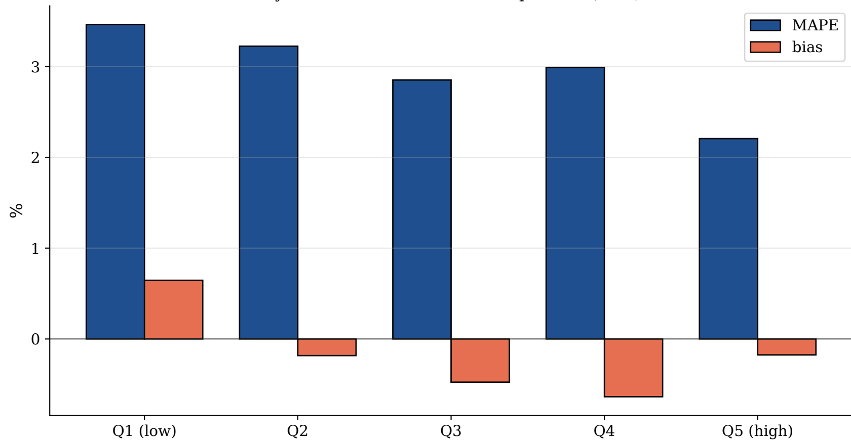
Hybrid calibration across cost quintiles (OOF)
