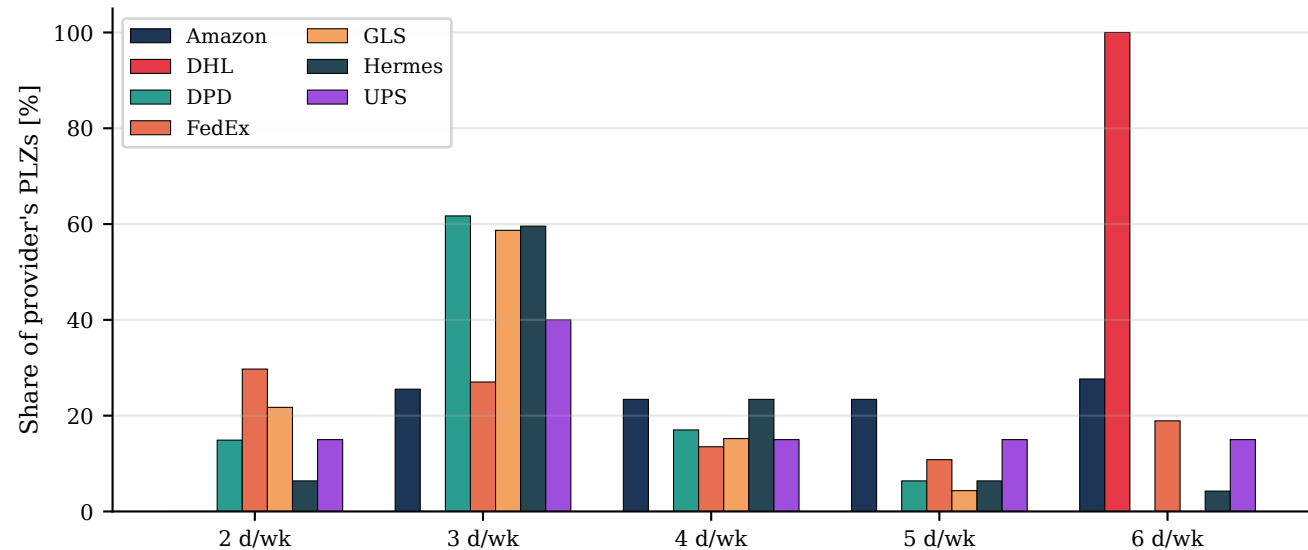
Per-provider frequency histogram at P = 0.5 , \theta = 1
