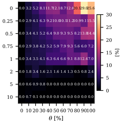
(c) Peak-fleet reduction [%]
