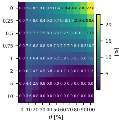
(b) Cost saving, fleet-balanced [%]
