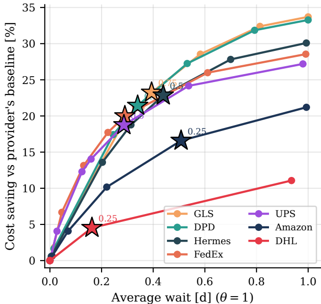
(a) Per-provider Pareto fronts with knees
