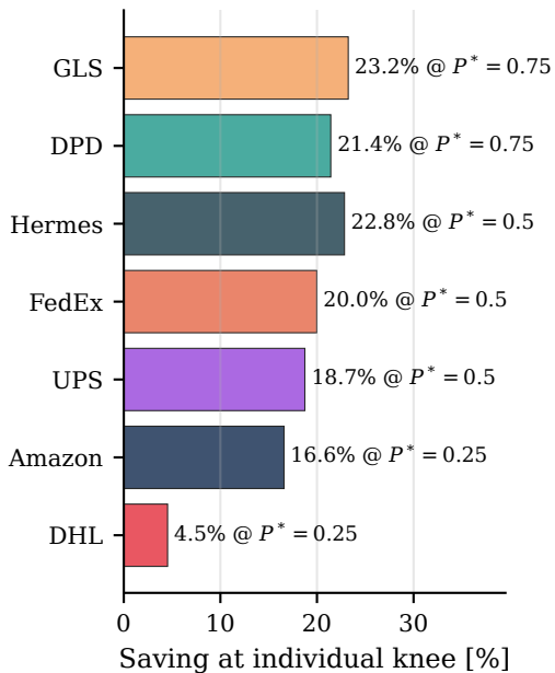
(b) Individual sweet-spots
