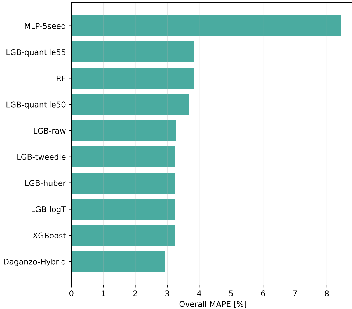
Overall accuracy
