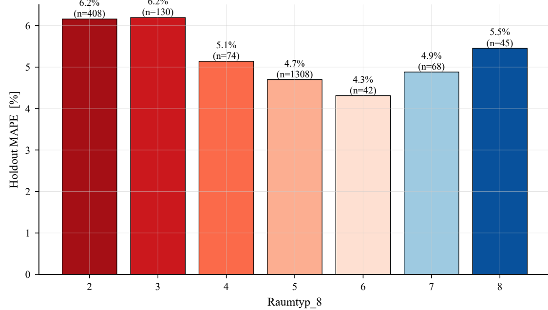
(b) Surrogate-Quality je Raumtyp_8
