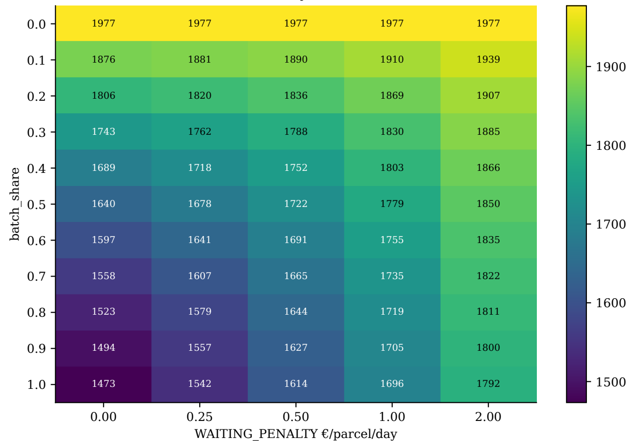
Total weekly cost [k€]
