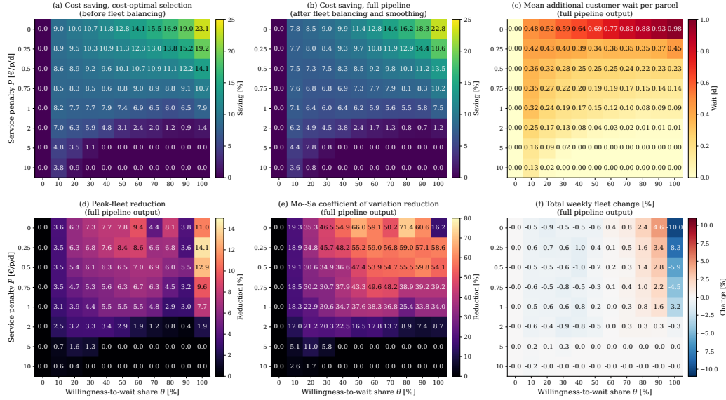
Figure 5: Total cost saving (a, b), parcels-weighted additional customer wait (c), and fleet metrics (d-f) over the service-penalty P and willingness-to-wait \theta grid, reported relative to the daily-delivery baseline.
