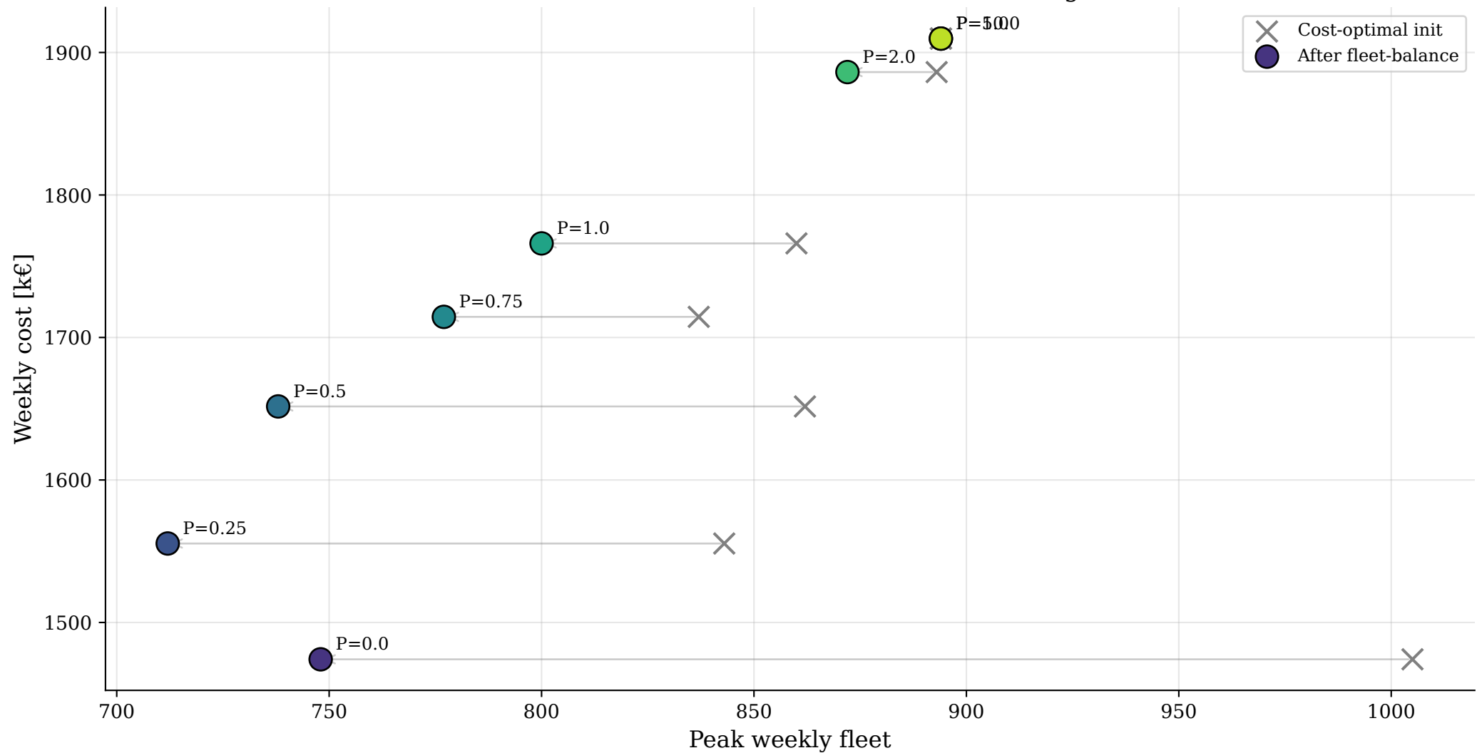
Cost-Fleet trade-off at share=100% — fleet balancing arrows
