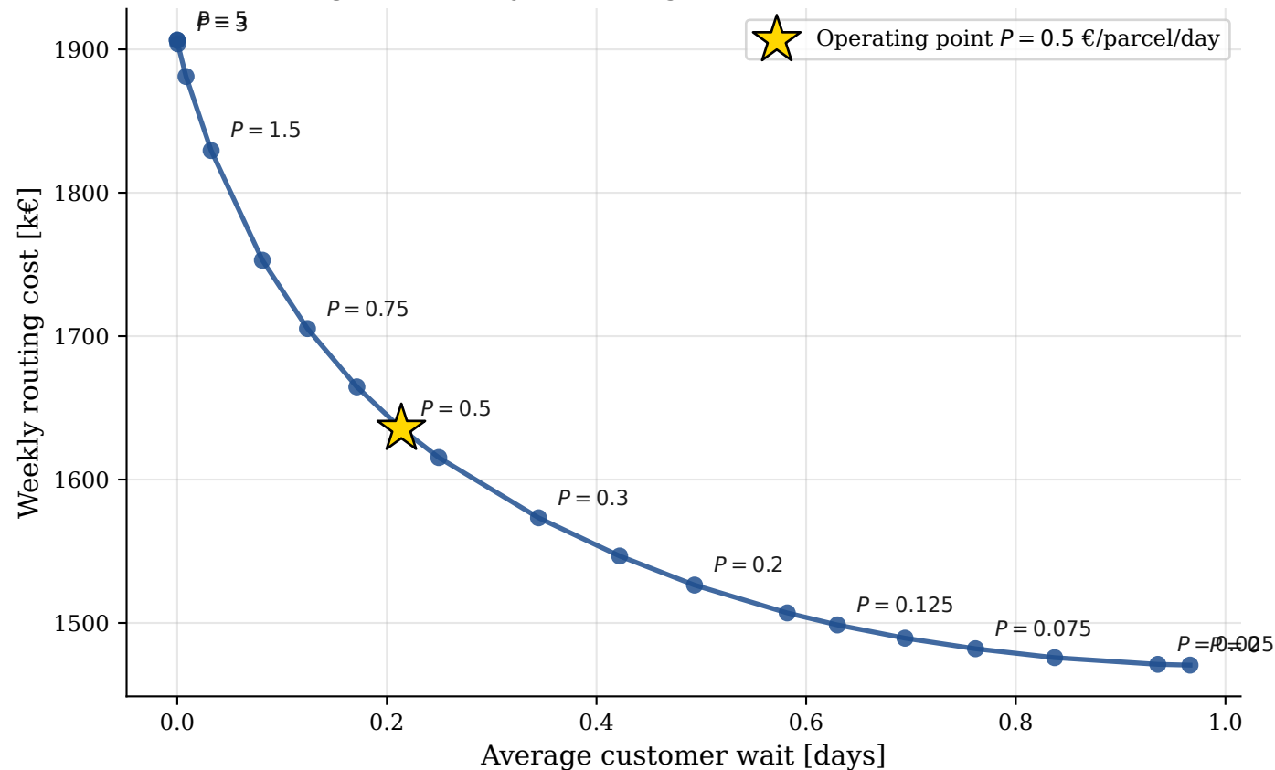
Service-cost Pareto frontier: penalty sensitivity (Daganzo-LGB-Hybrid surrogate, 312 (provider, PLZ) cells)
