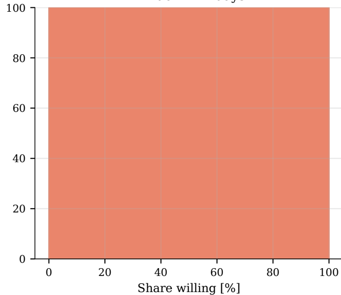
window = 1 days
