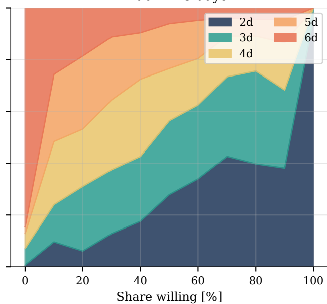
window = 3 days
