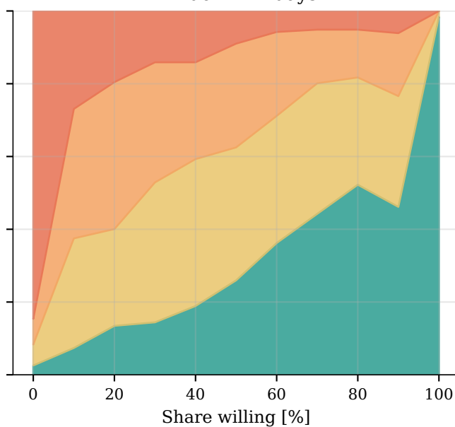
window = 2 days
