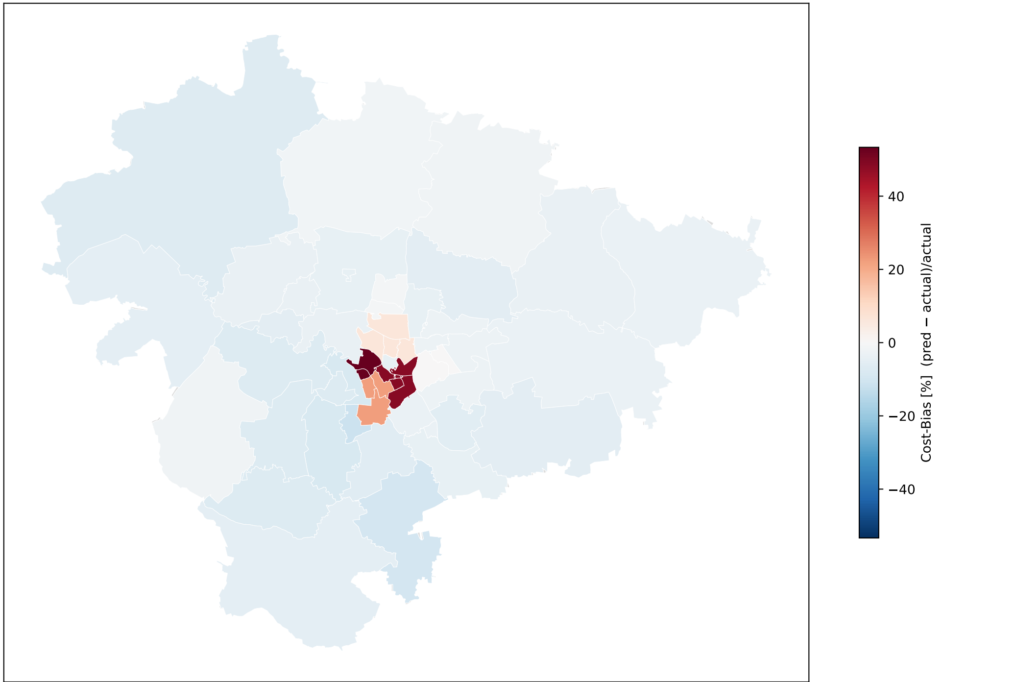
Fig MLA3 — LGB-logT signed cost-bias per cluster Blue = model underestimates cost; Red = overestimates. White = unbiased.
