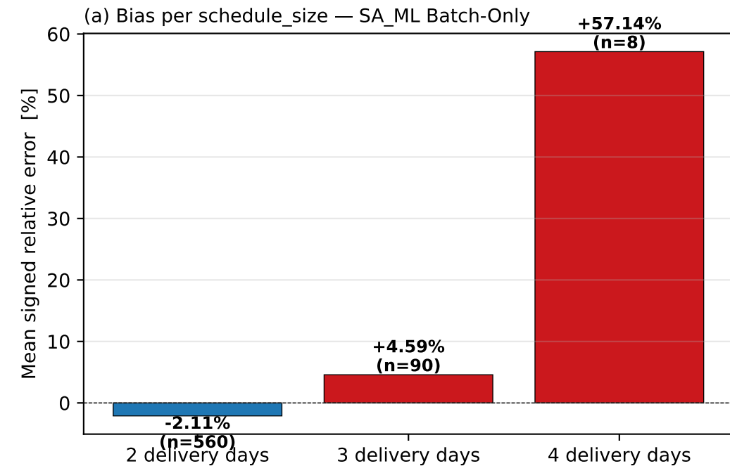
Fig PQ2 — Per-schedule-size error decomposition (out-of-pool optimizer-chosen)
