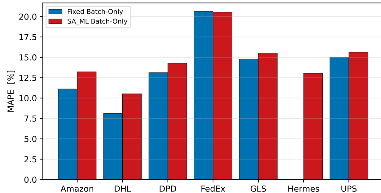
(a) Cost-MAPE per Provider × Scenario
