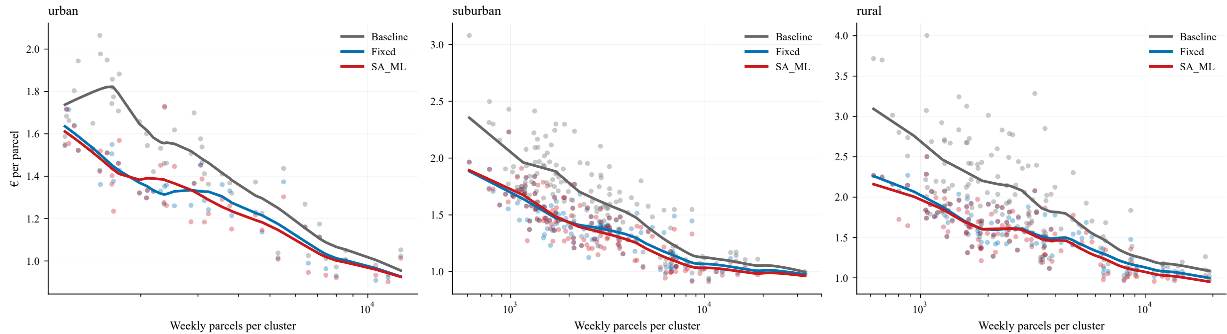
Fig S2 — Cost per parcel: Baseline / Fixed / SA_ML vs. weekly volume
