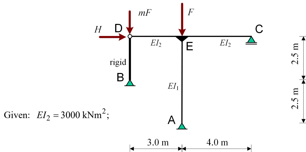
Figure 1 : Frame loaded with concentrated forces
