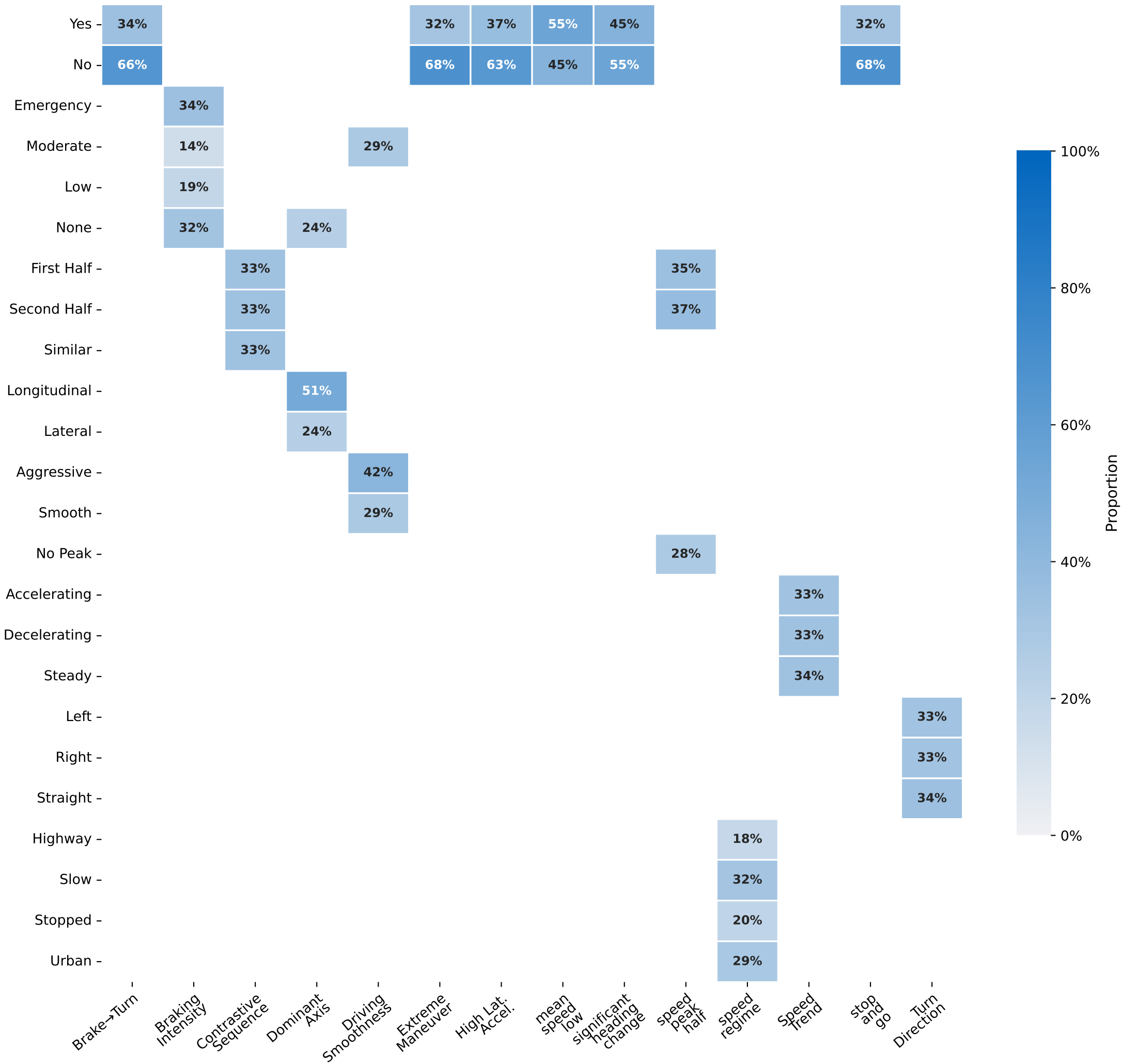
Answer Distribution Across Question Types
