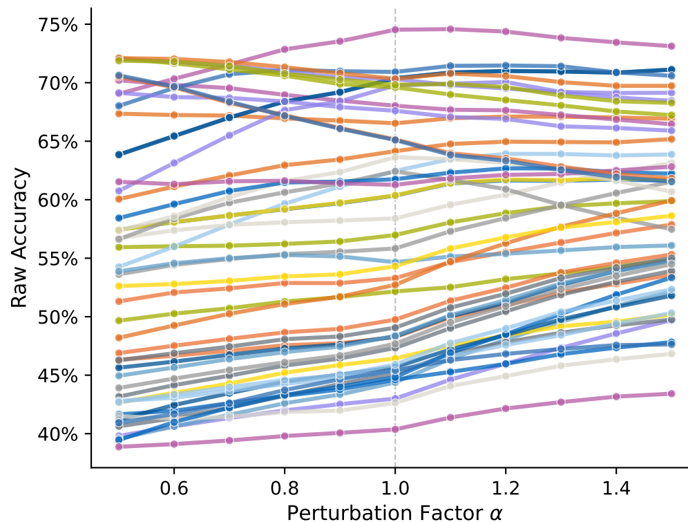
Raw Accuracy
