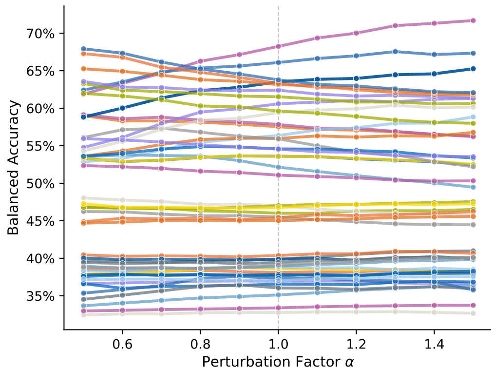
Balanced Accuracy
