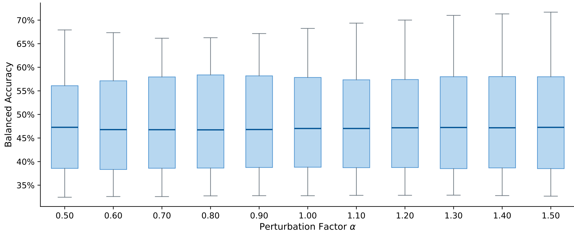
Distribution of Model BAcc across Perturbations
