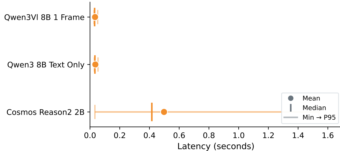
Per-Request Latency Distribution (NVIDIA GeForce RTX 5090)
