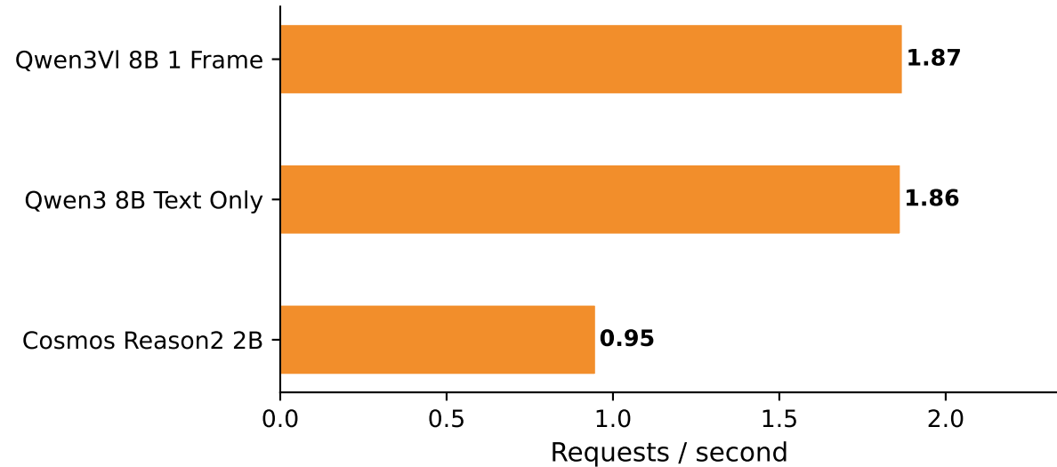
Throughput (NVIDIA GeForce RTX 5090)
