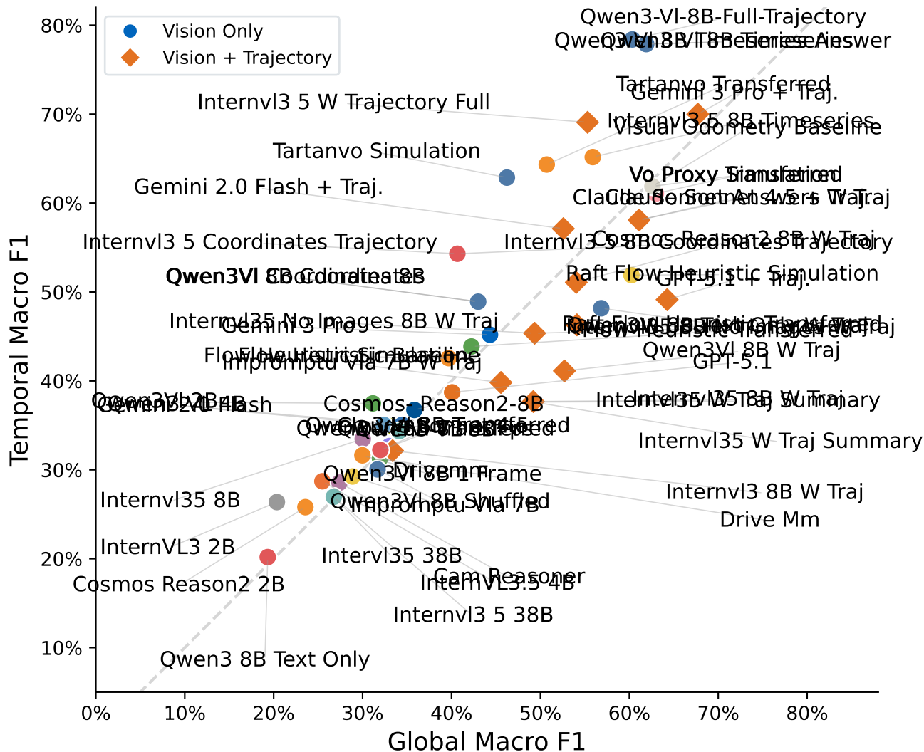
Global vs. Temporal Reasoning
