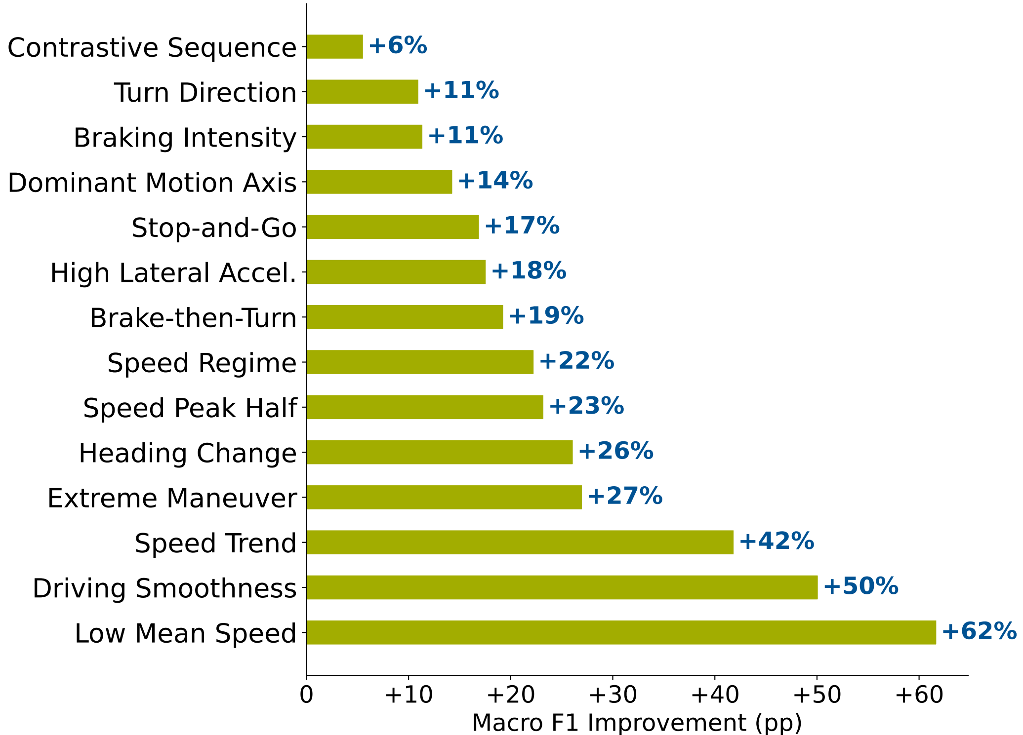
Trajectory Feature Impact — Gemini 3 Pro
